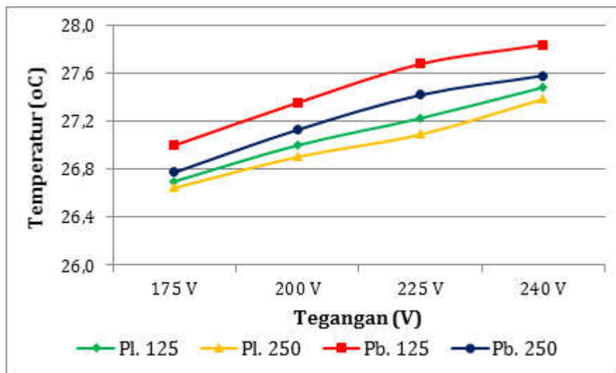
Gambar 5. Temperatur air
